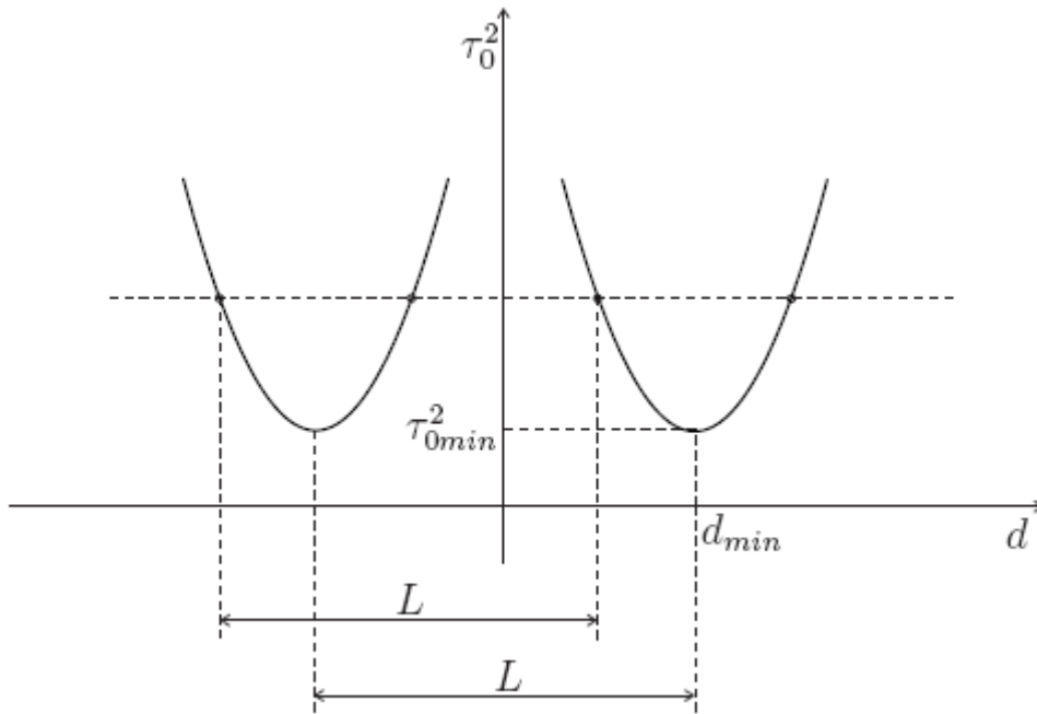
Fig. 2 Dependence of the square of the swing time on the distance d
