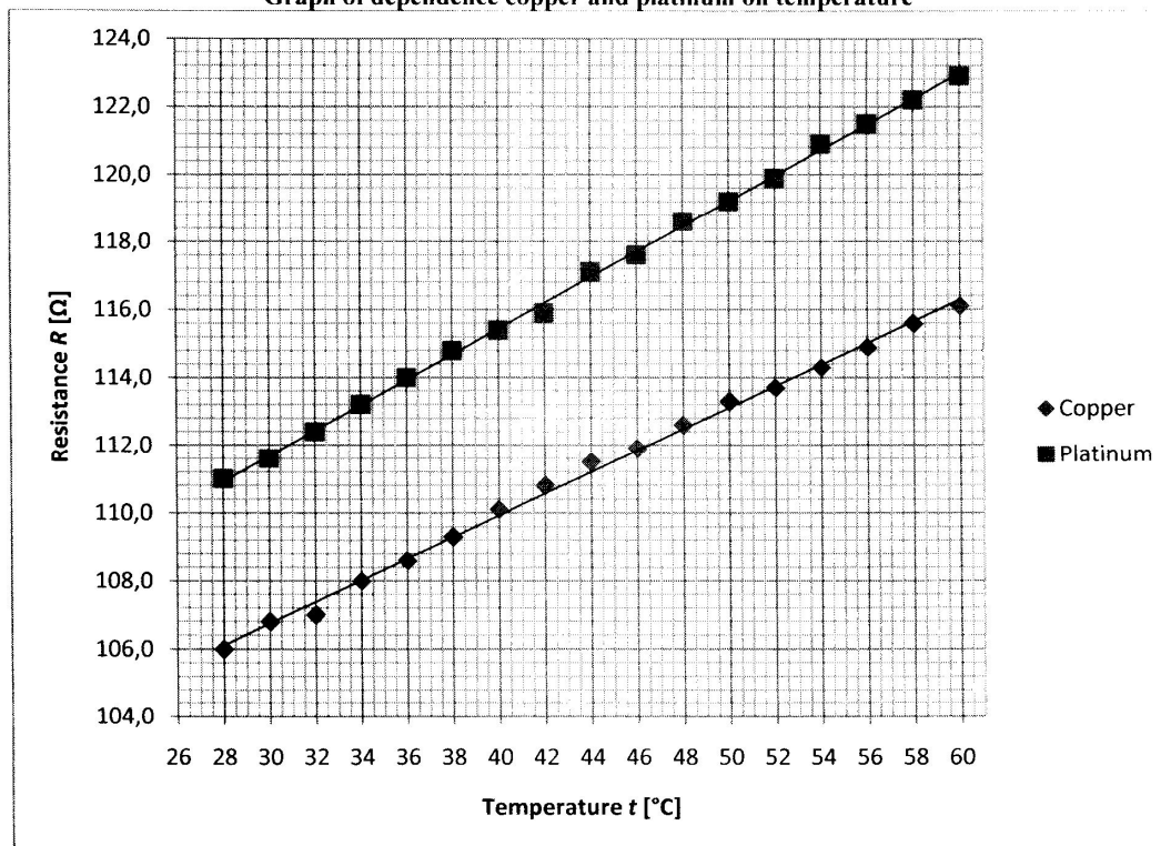
Graph of dependence copper and platinum on temperature
